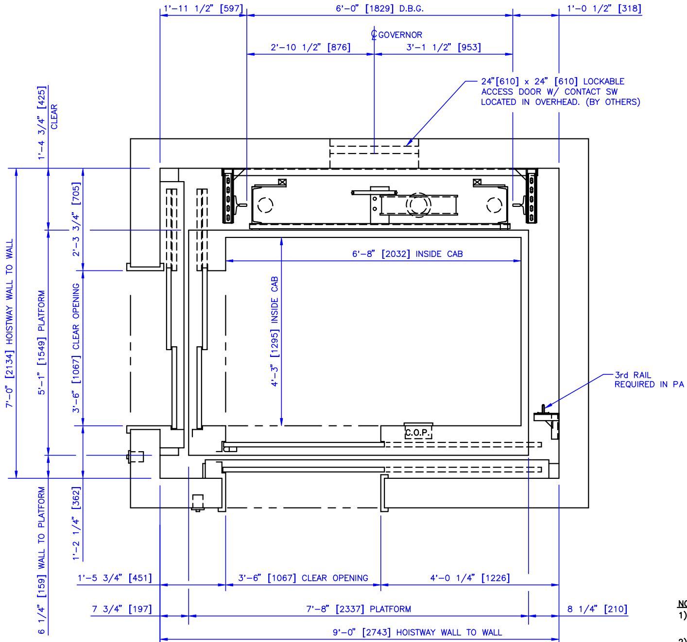
HOISTWAY PLAN 2500# [1130 KG] CAPACITY UP TO 90'-0" [27432] OF TRAVEL (HIGHER TRAVELS POSSIBLE, CONSULT FACTORY)
