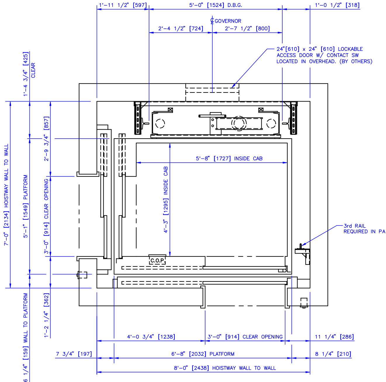
HOISTWAY PLAN 2000# [905 KG] CAPACITY UP TO 90'-0" [27432] OF TRAVEL (HIGHER TRAVELS POSSIBLE, CONSULT FACTORY)
