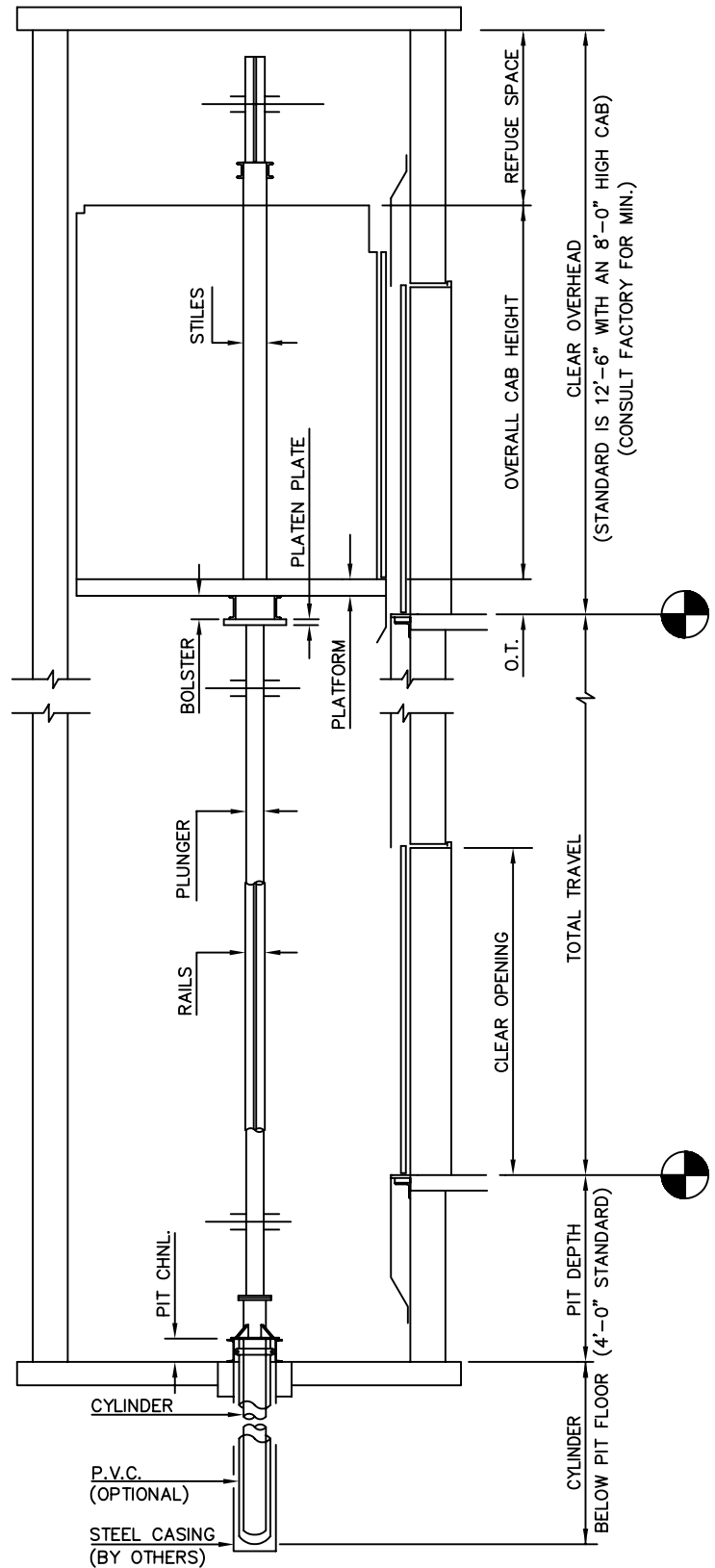
SECTION
