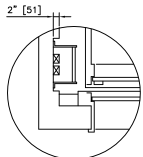
HOISTWAY NOTCH FOR PIT LADDER – 2002 CODE
