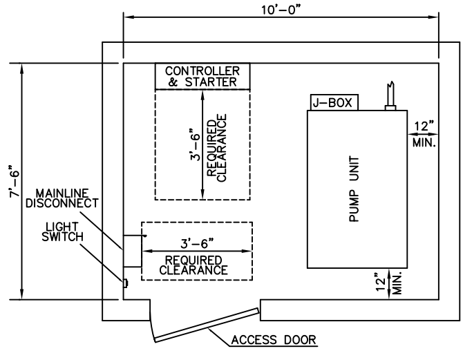
MACHINE ROOM #1
