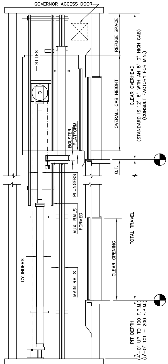
SECTION
